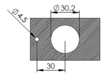
PANEL APERTURE
