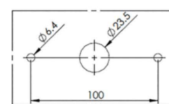
PANEL APERTURE
